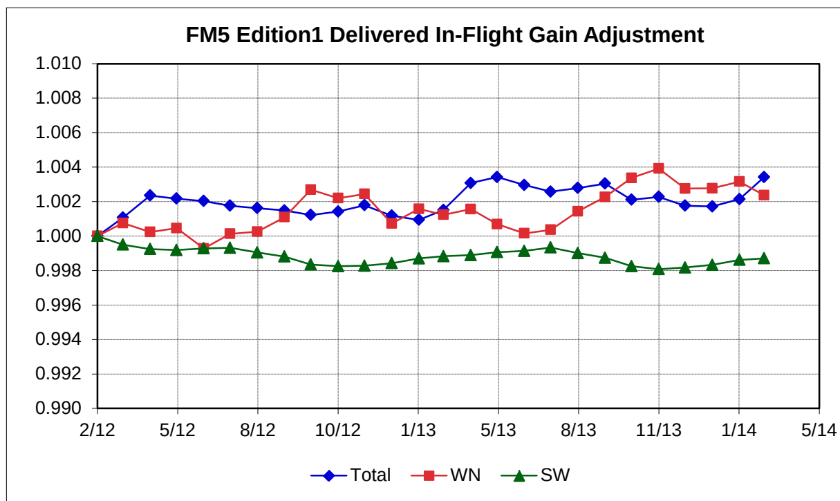
Figure 2-1 FM 5 Edition 1 In-Flight Gain Adjustment
